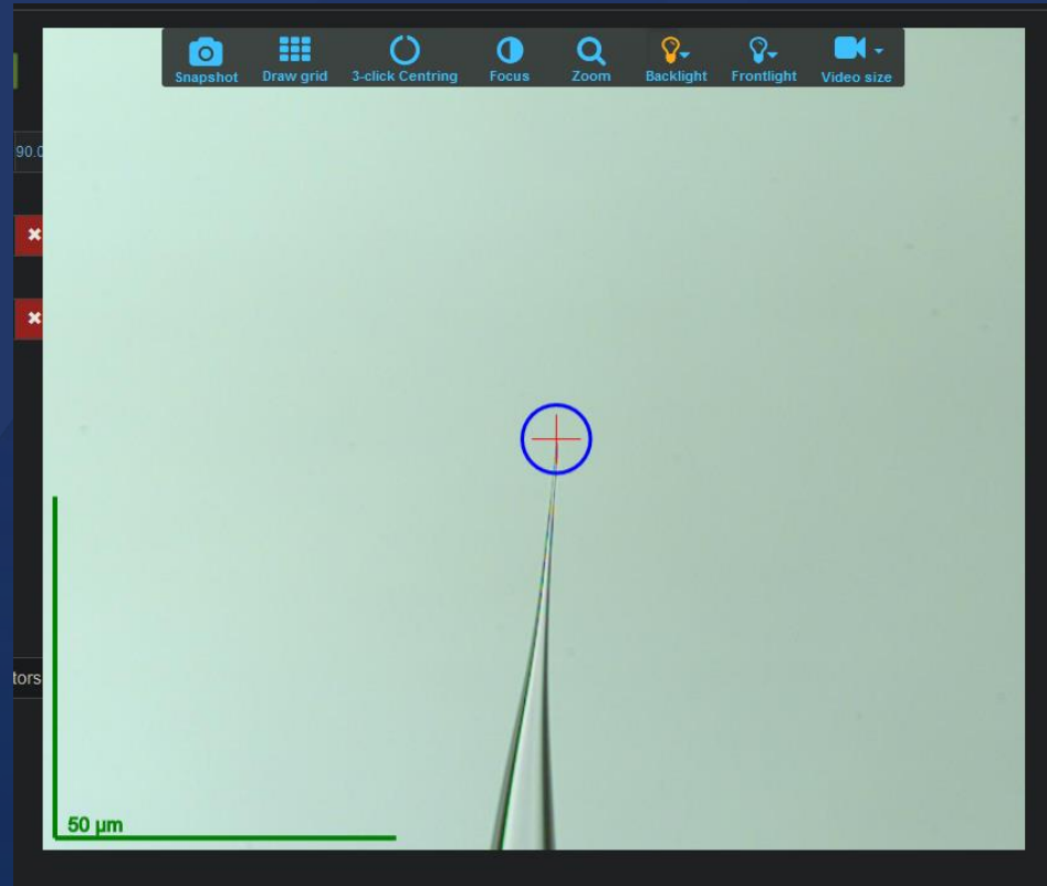
Testing the precision of our automatic loop alignment – the glass capillary test object tapers off to a 2µm point.
