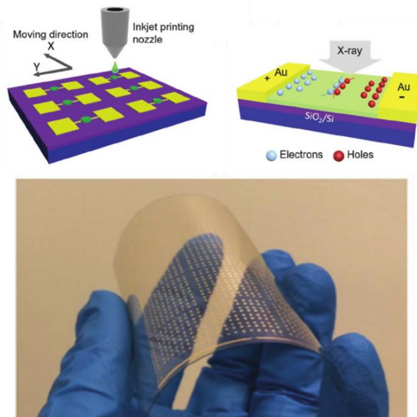
Schematic of the inkjet printing method and detection of x-rays (top), for a flexible array of X-ray detectors based on novel \text{CsPbBr}_3 quantum dots
