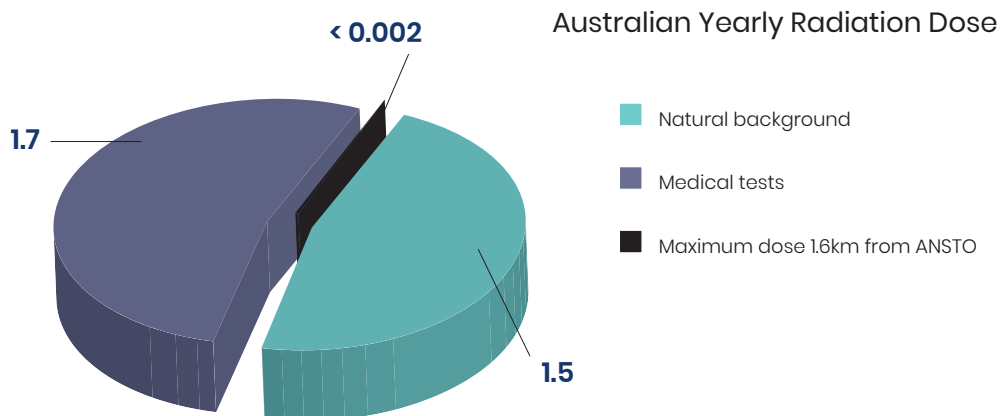
Figure 2: The average annual dose received by Australians from various sources compared to the maximum potential airborne dose to ANSTO's nearest residents in 2017-2018. *Source: ARPANSA Fact Sheet http://www.arpansa.gov.au/pubs/factsheets/IonisingRadiationandHealth.pdf
